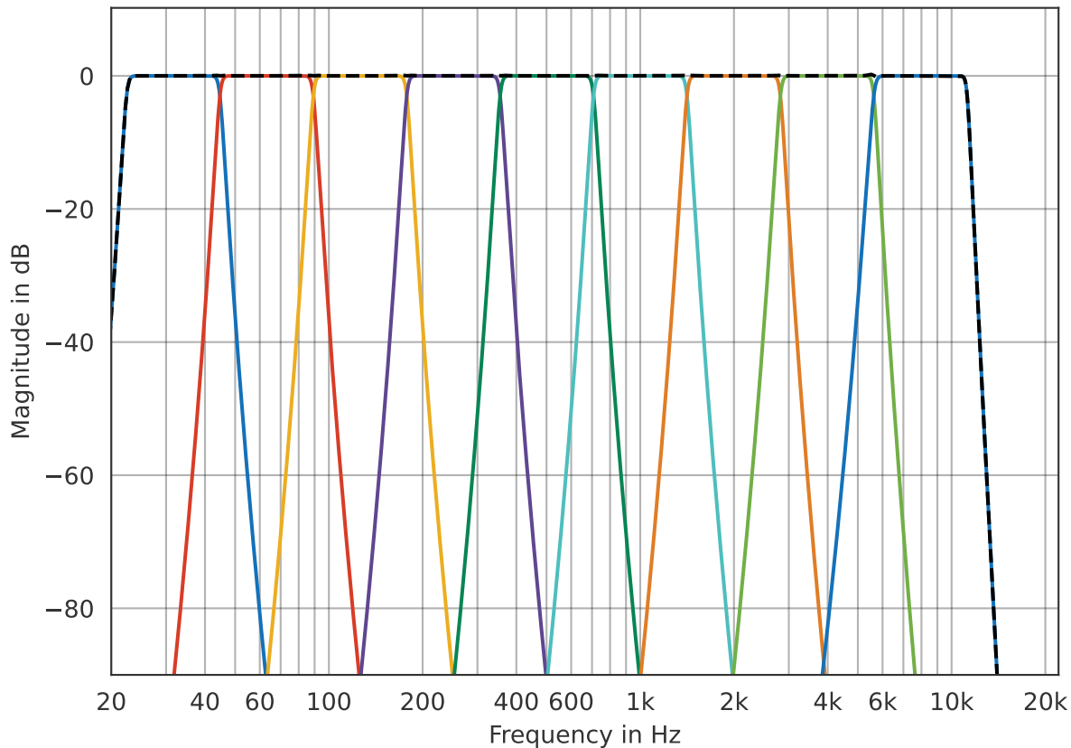
Filter bands and the sum of their squared magnitudes
