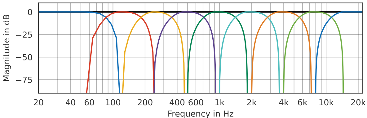
Reconstructed (black) and filtered impulse (colored)
