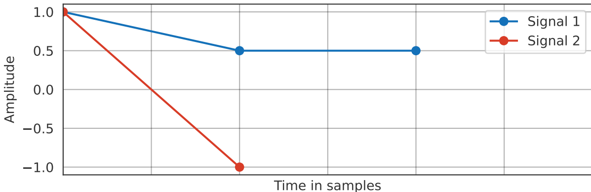
Convolution Result
