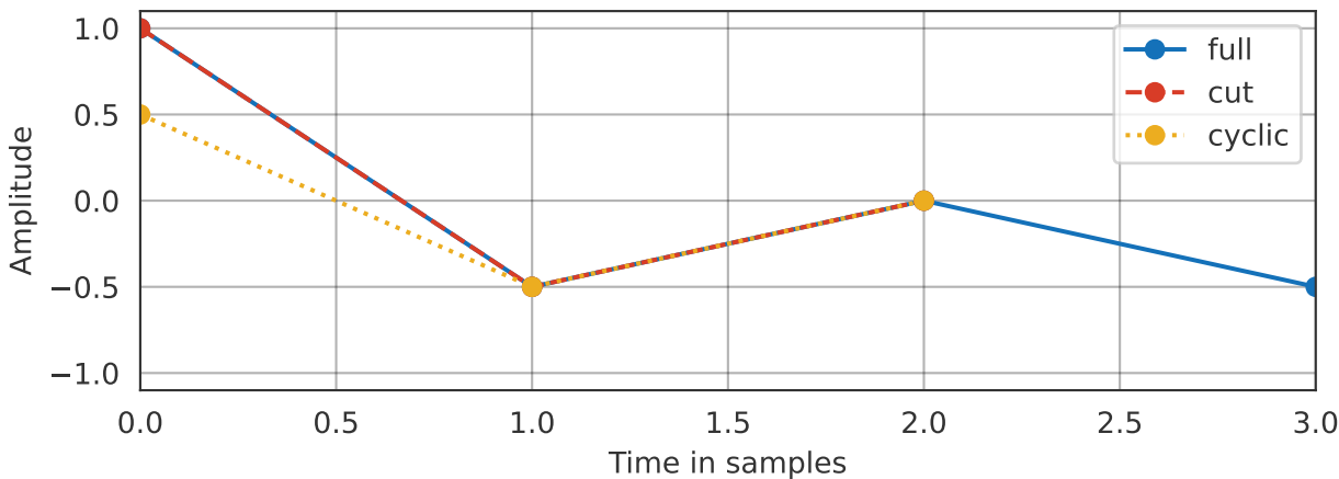
Convolution Result
