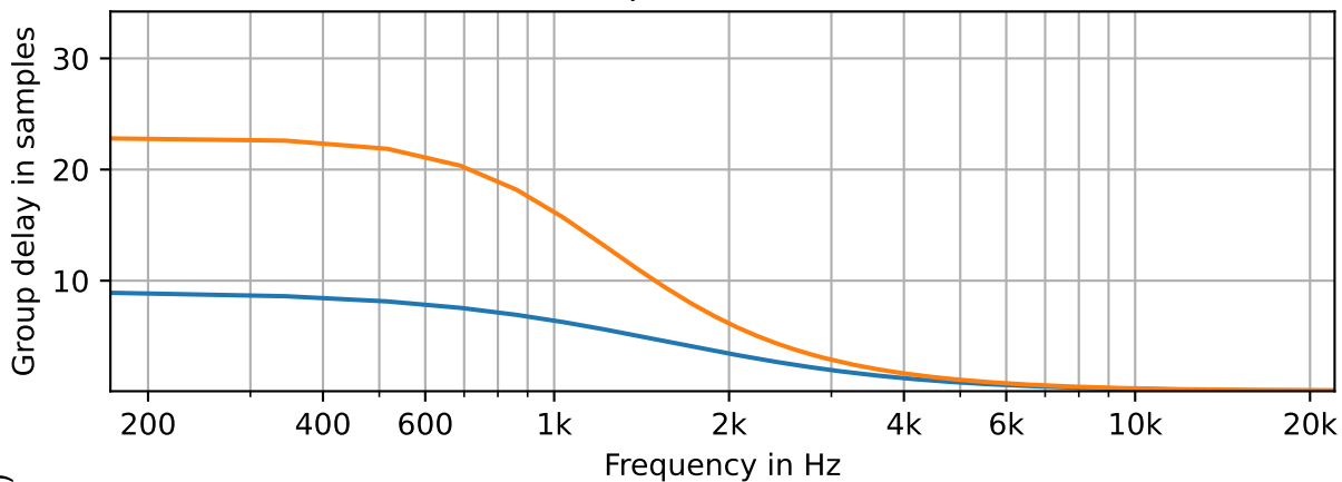
1. and 2. order allpass filter with f_c = 1000 Hz
